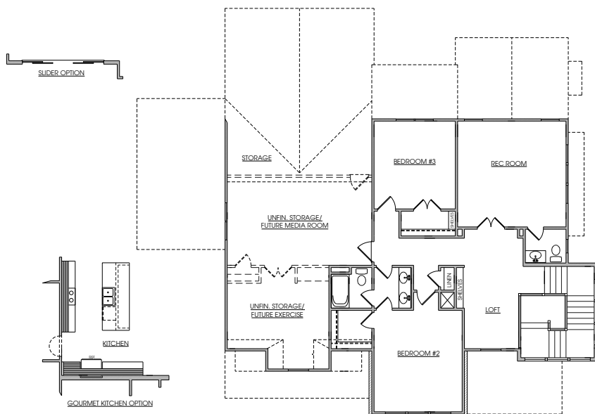
SECOND FLOOR
